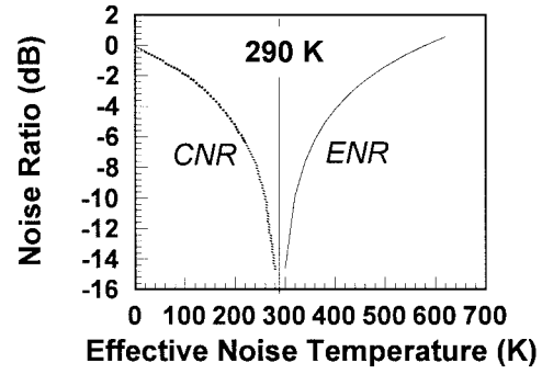
Fig. 3. Functional behavior of CNR and ENR in the neighborhood of 290 K.
