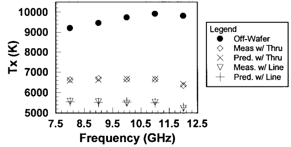
Fig. 4. Comparison of measured and predicted on-wafer temperature (at plane 7 of Fig. 1) presented by a coaxial diode noise source connected to Probe 2. Measurements were made with both a short (thru) and long (line) CPW line connected between the probes.
