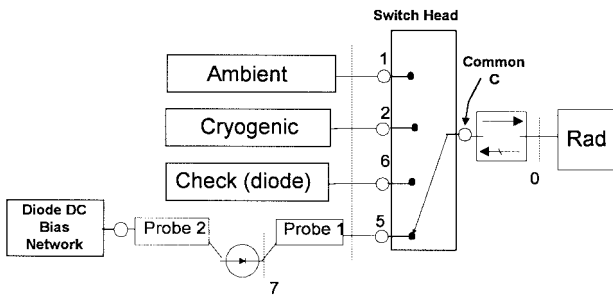
Fig. 2. Configuration for characterization of on-wafer diode noise sources. Bias is applied through Probe 2.
