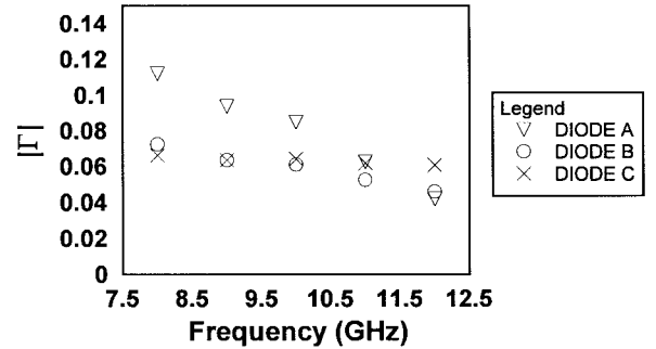
Fig. 10. Reflection-coefficient magnitudes for the three on-wafer diode noise sources with dc bias on.
