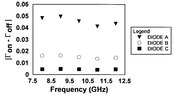
Fig. 11. Magnitude of vector difference between reflection coefficients of bias-on and bias-off diodes.
